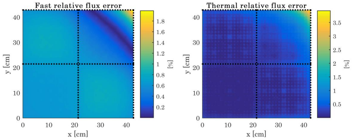
Figure 12. Within-core fast and thermal relative error profiles for the C5G7 core with one core sweep re-homogenization
